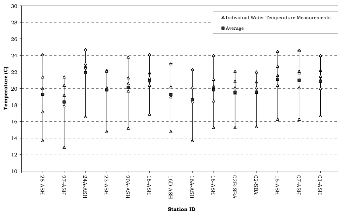
Figure 5. Water Temperature Statistics for the Ashuelot River Watershed May 25 - September 14, 2010, NHDES VRAP
