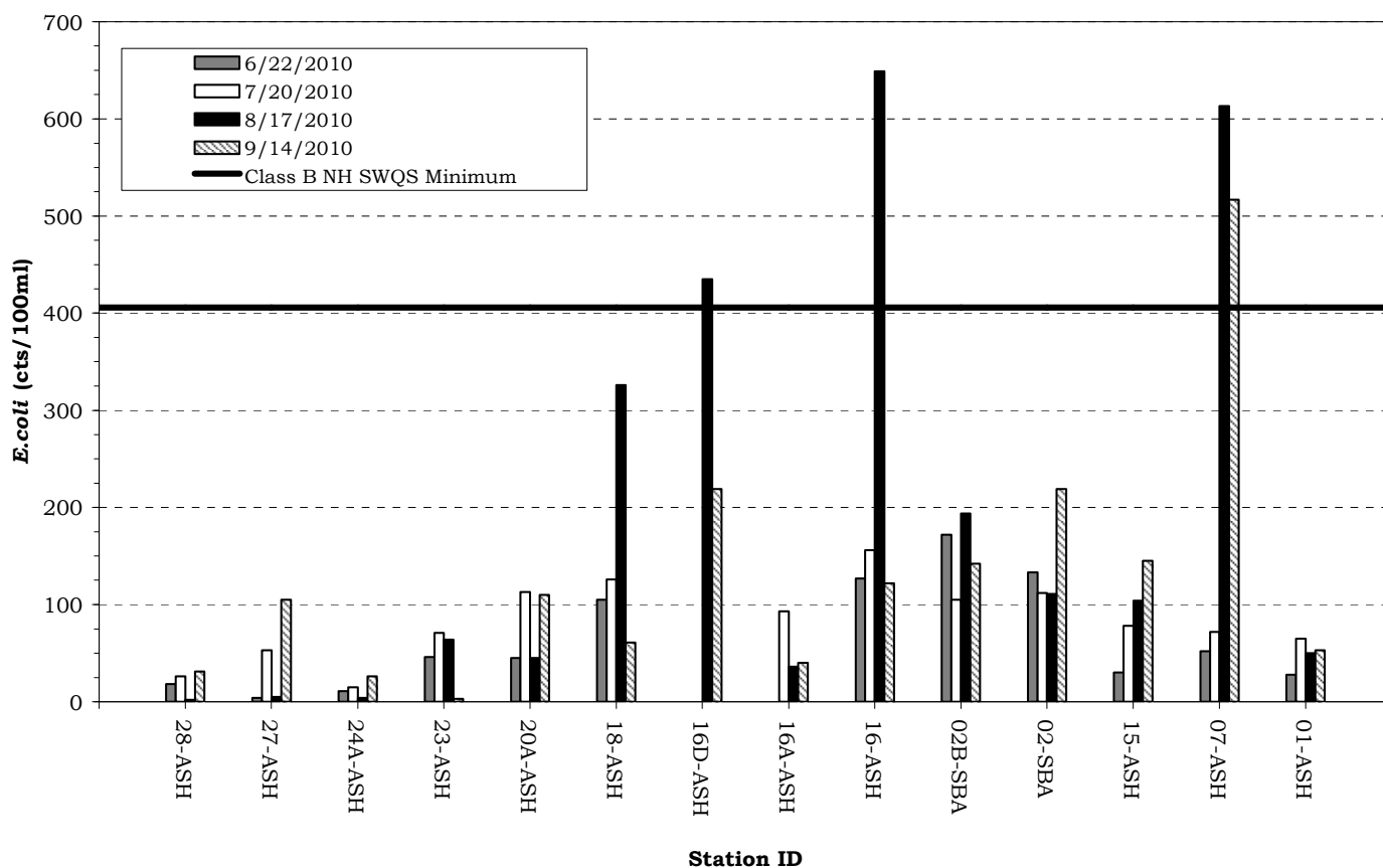
Figure 6. Escherichia coli Statistics for the Ashuelot River Watershed June 22 - September 14, 2010, NHDES VRAP
